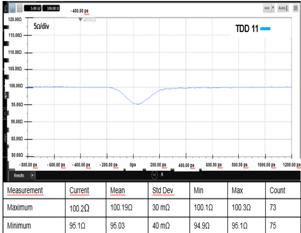
Figure 15: TDR measurement
