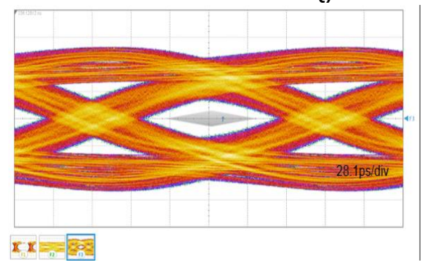
Figure 7: Eye diagram - HDMI 2.0 mask at 5.94 Gbps per channel (with HSP051-4N10, with worst case reference cable and EQ)
