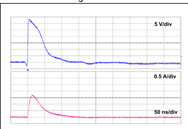
Figure 14. Response to ISO 7637-3 (pulse 3b) U_S = +100 V
