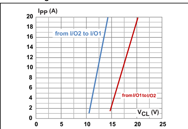
Figure 10. TLP measurements
