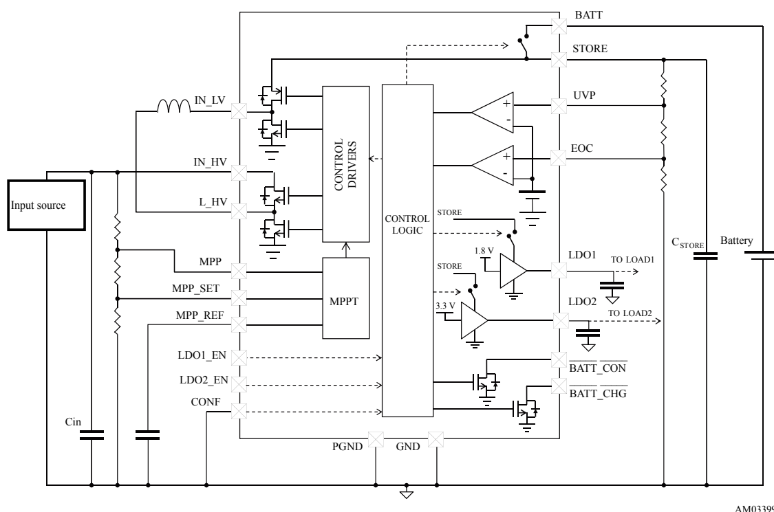
Figure 12. Buck-boost configuration example
