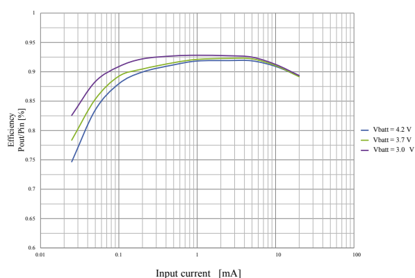
Figure 11. Efficiency vs. input current; V_{OC} = 2.5 V
