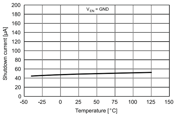
Figure 13: Shutdown current vs. temperature
