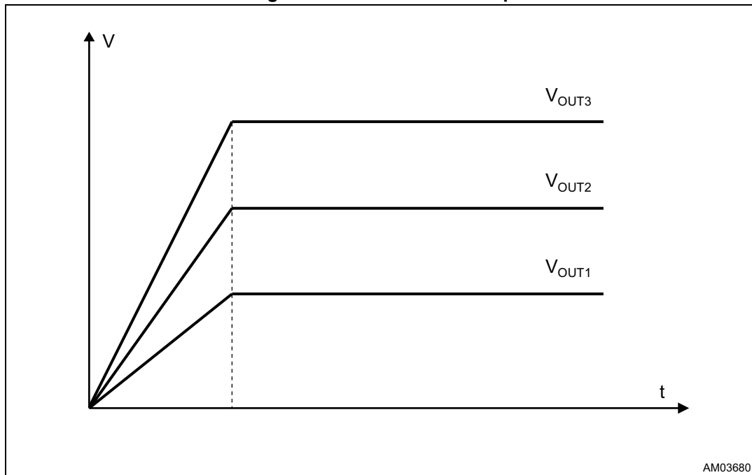
Figure 10. Ratiometric startup
