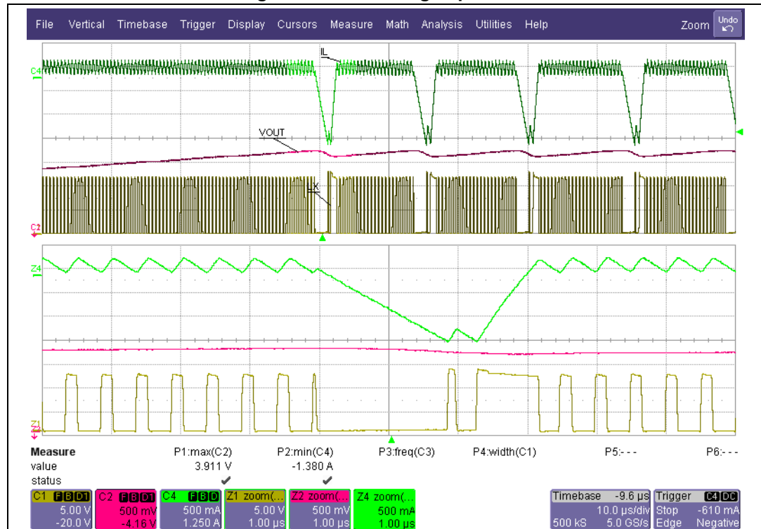
Figure 23. Overvoltage operation
