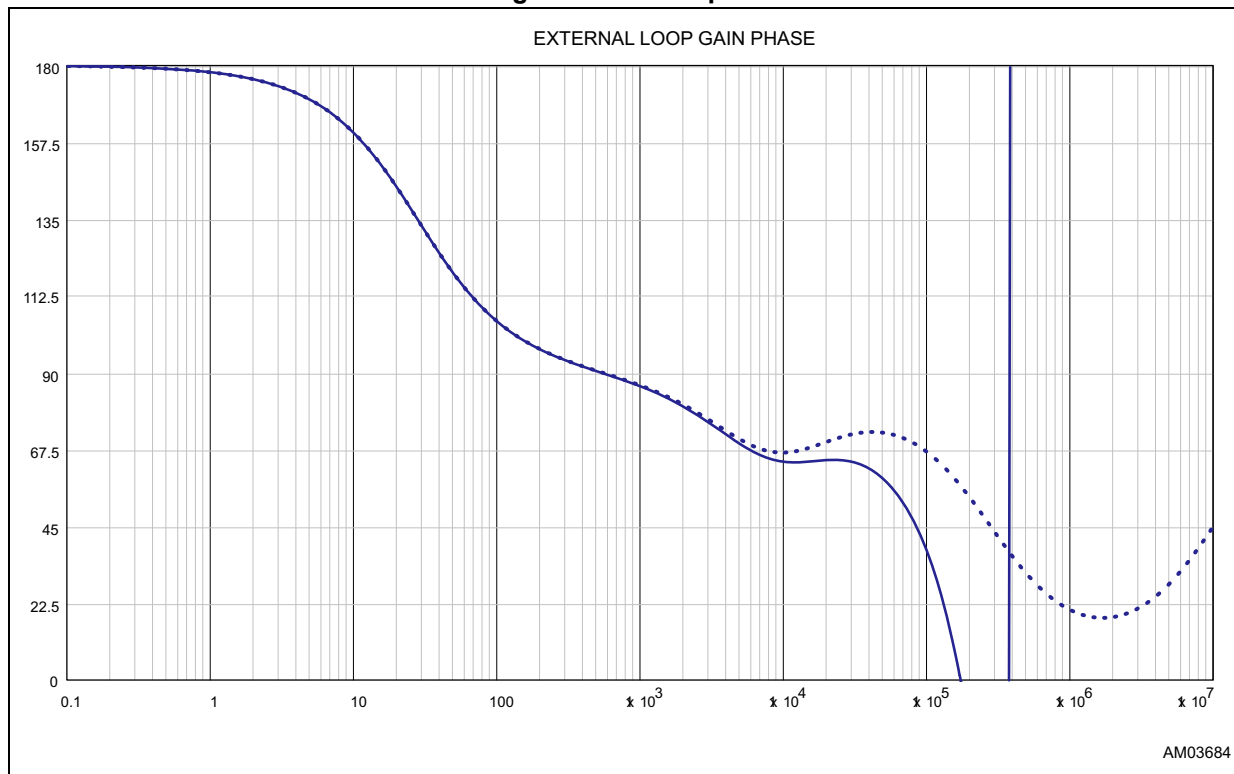
Figure 28. Phase plot
