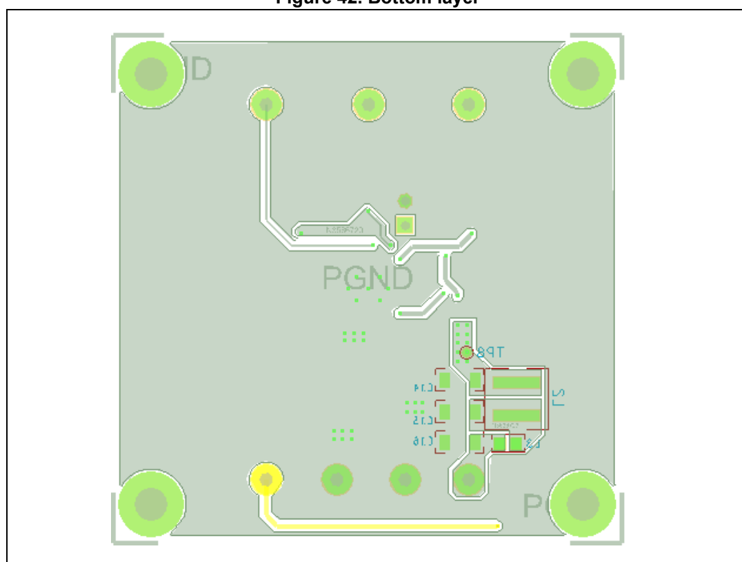
Figure 42. Bottom layer
