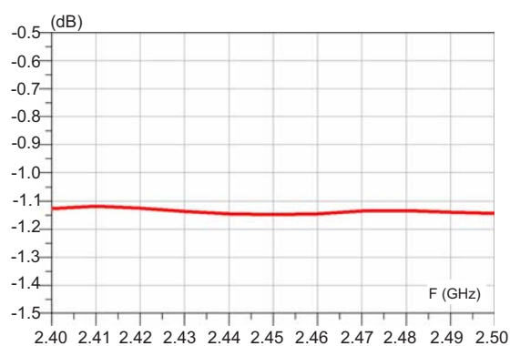
Figure 4. Insertion loss ( T_{amb} = 25\text{ °C} )
