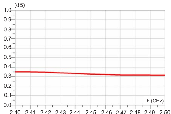
Figure 6. Amplitude imbalance ( T_{amb} = 25\text{ °C} )
