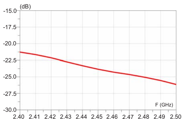
Figure 3. Return loss ( T_{amb} = 25\text{ °C} )
