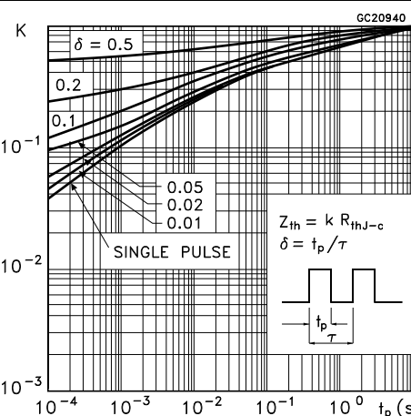
Figure 7. Thermal impedance for TO-220
