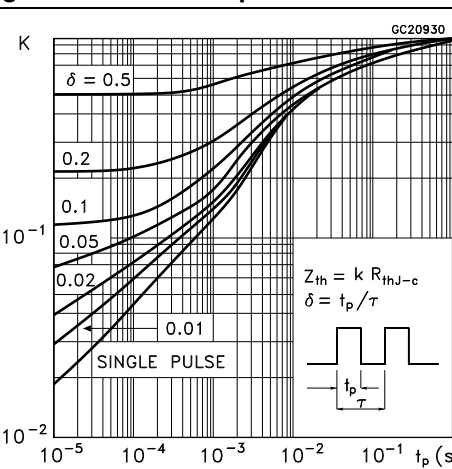
Figure 7. Thermal impedance for TO-220
