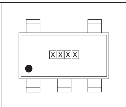
Figure 8. Marking layout
