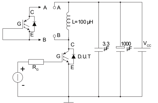
Figure 33. Test circuit for inductive load switching
