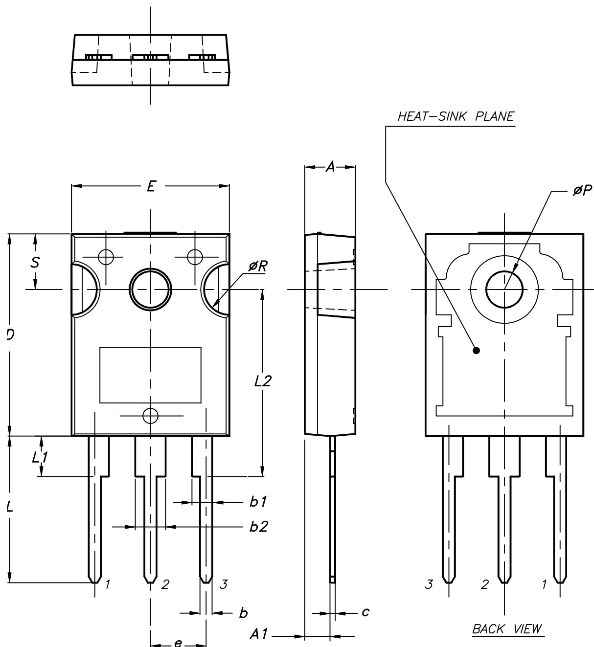
Figure 38. TO-247 package outline
