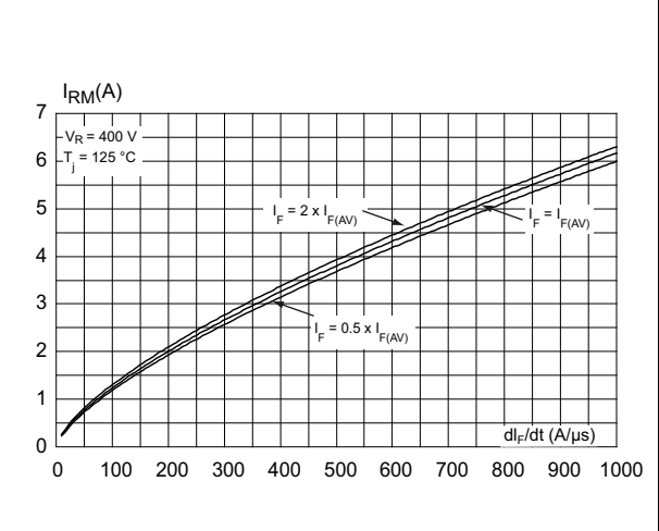
Figure 4. Peak reverse recovery current versus di_F/dt (typical values)
