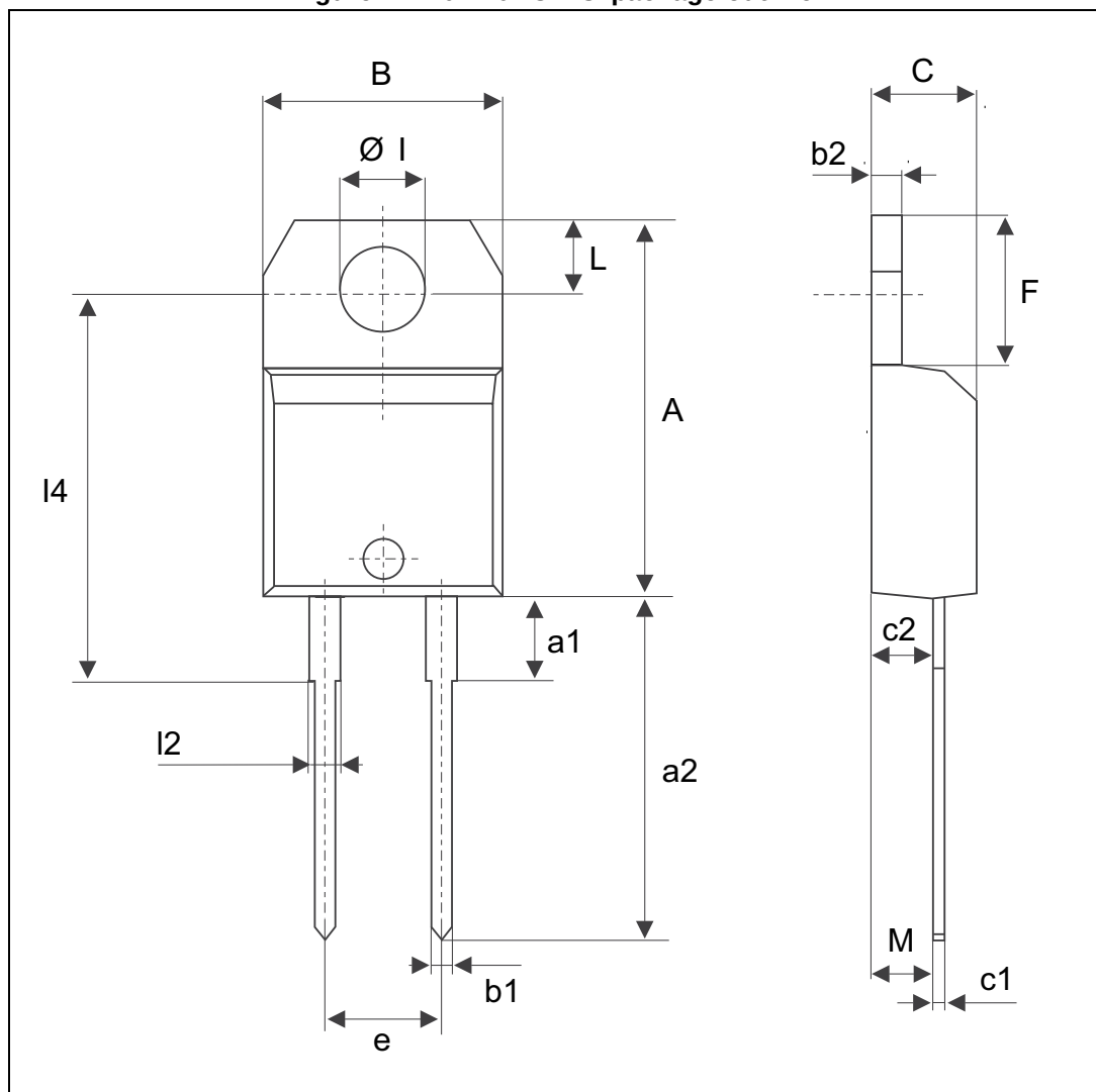
Figure 12. T0-220AC ins. package outline
