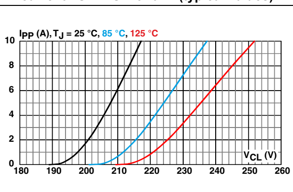
Figure 7. Clamping voltage versus peak pulse current - STRVS225X02E (typical values)
