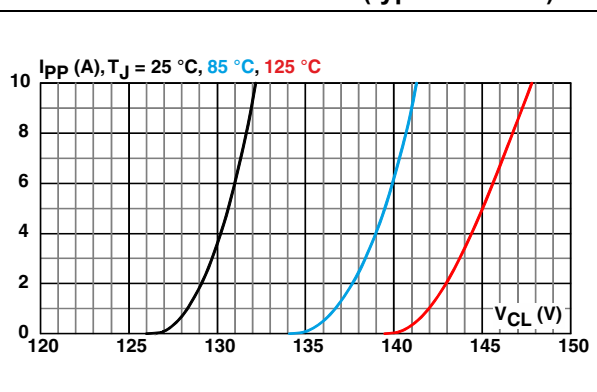
Figure 3. Clamping voltage versus peak pulse current - STRVS142X02F (typical values)
