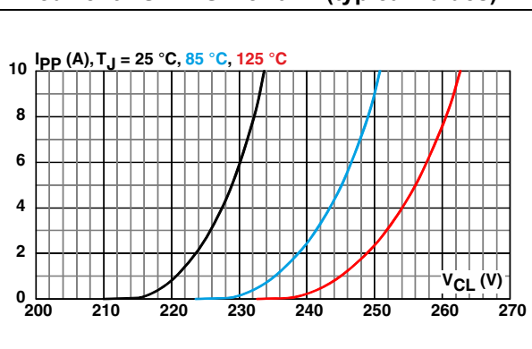
Figure 9. Clamping voltage versus peak pulse current - STRVS248X02C (typical values)
