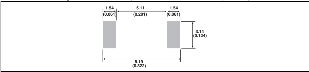
Figure 24. SMC footprint, dimensions in mm (inches)
