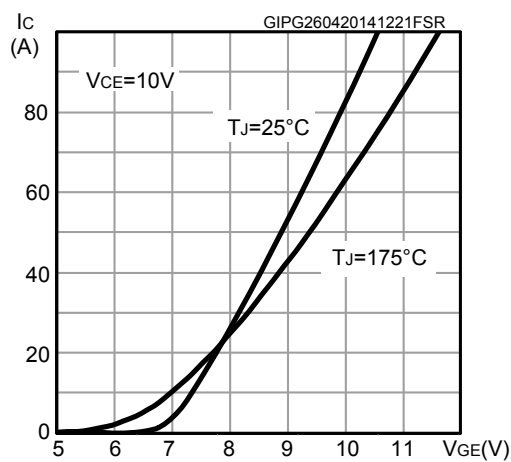
Figure 9. Transfer characteristics
