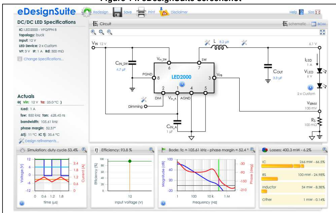
Figure 14. eDesignSuite screenshot
