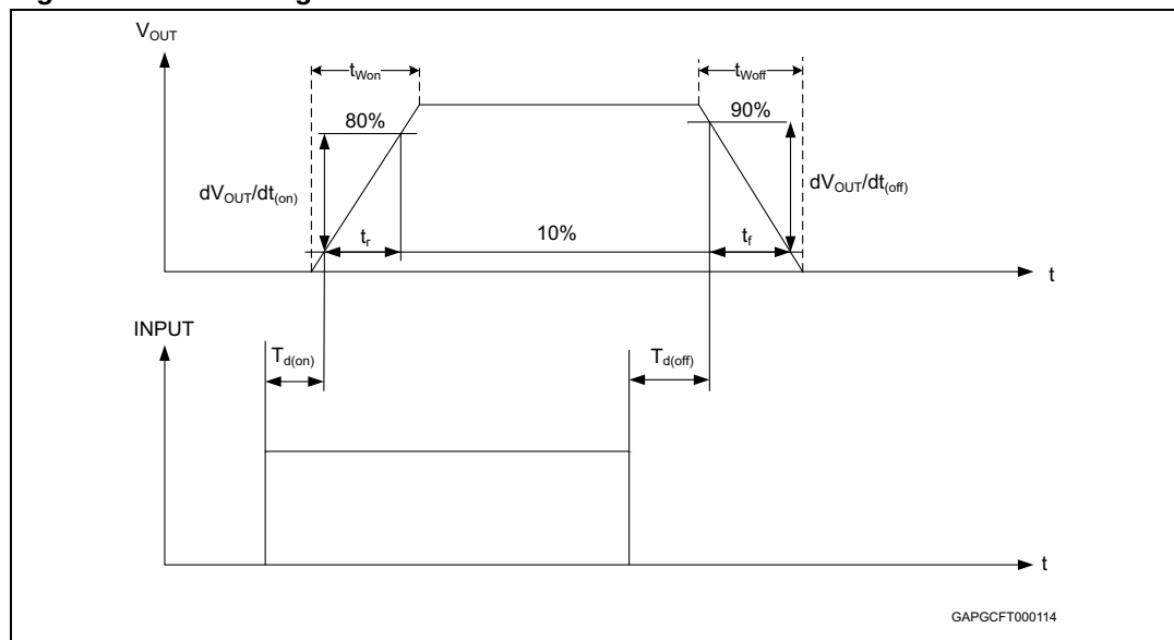
Figure 8. Switching characteristics
