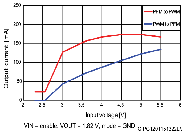
Figure 10: Mode transition vs. input voltage
