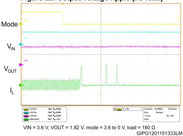
Figure 12: Output voltage ripple (no-load)
