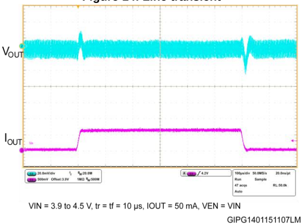
Figure 14: Line transient
