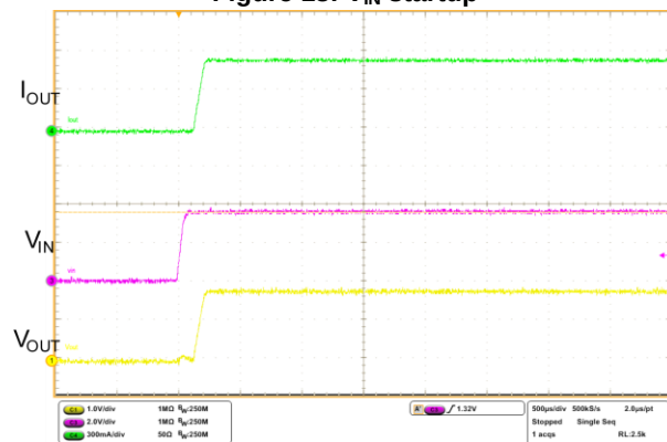
Figure 18: V_{IN} startup
