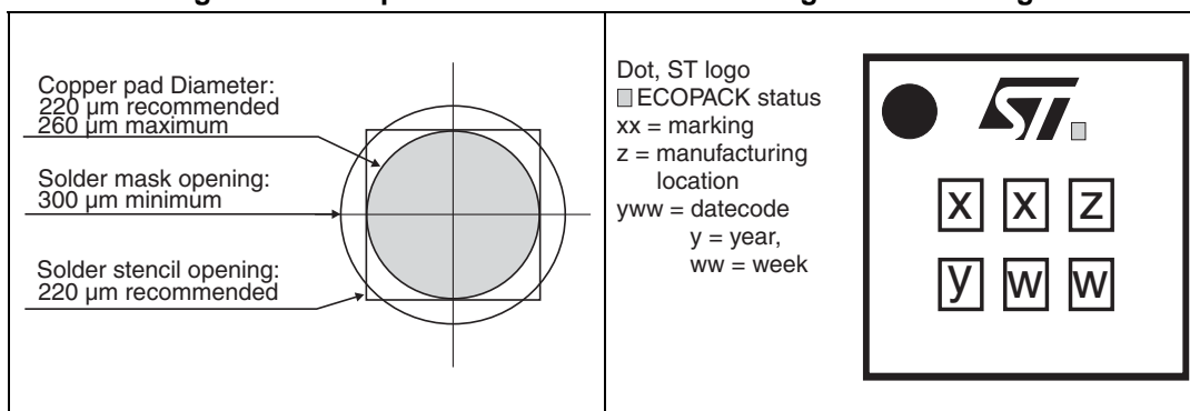
Figure 10. Footprint
