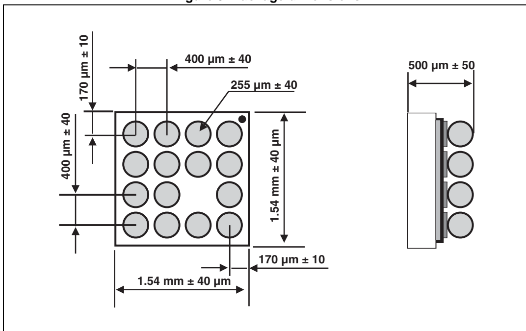
Figure 9. Package dimensions
