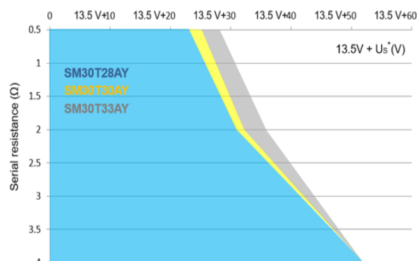
Figure 18. Load dump capability (typical values, U_S^* = f(R_i) pulse 5b, U_S = 87\text{ V} , t_p = 150\text{ ms} )
