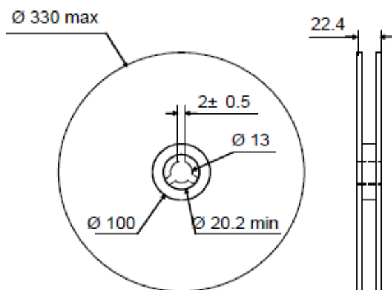
Figure 28. 13" reel dimension values (mm)
