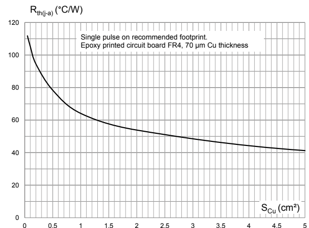
Figure 12. Thermal resistance junction to ambient versus copper area under each lead (SMC)
