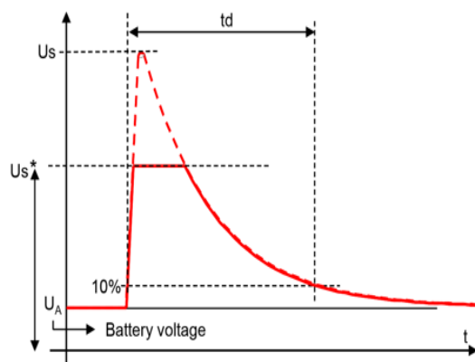
Figure 20. ISO16750-2 test B definition
