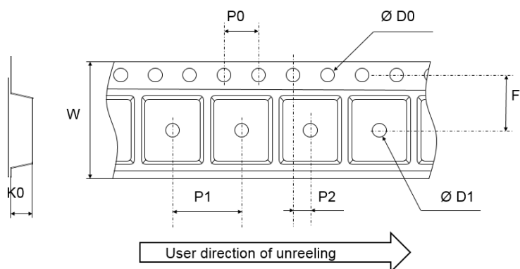
Figure 30. Tape outline
