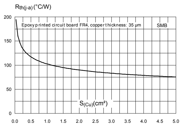
Figure 8. Thermal resistance junction to ambient versus copper surface under each lead (SMB)(typical values)
