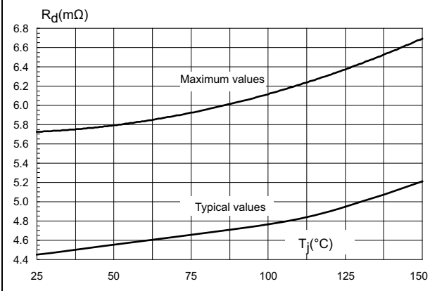
Figure 13. Dynamic resistance versus junction temperature
