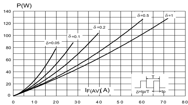
Figure 1. Conduction losses versus average current
