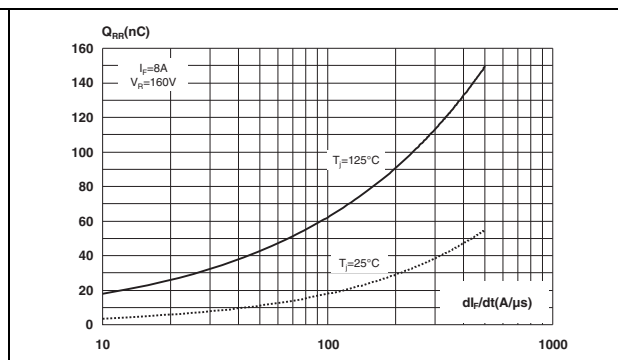
Figure 6. Reverse recovery charges versus di/dt (typical values)
