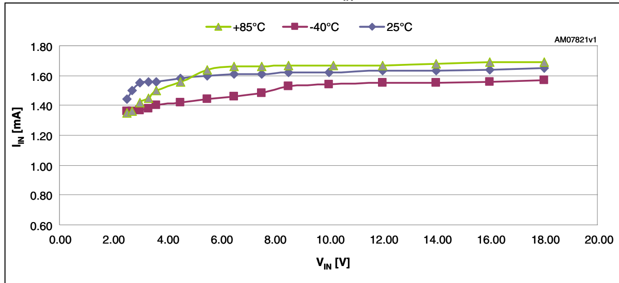
Figure 6. STLA02 driver current consumption vs. V_{IN}
