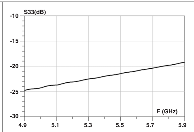
Figure 13. 5 G return loss ( T_{amb} = 25\text{ }^{\circ}\text{C} )
