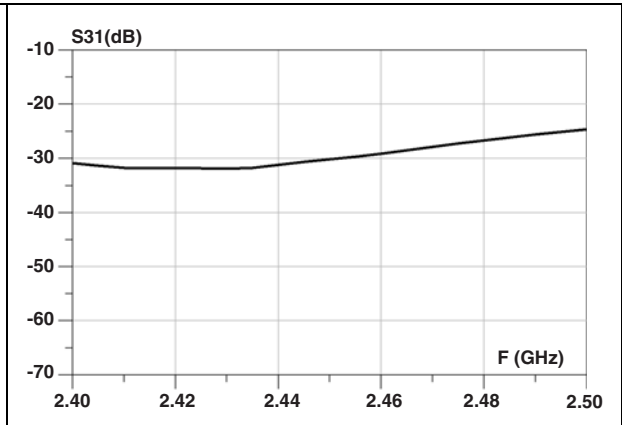
Figure 11. 5 G attenuation in 2 G band ( T_{amb} = 25\text{ }^{\circ}\text{C} )
