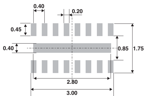
Figure 9. Footprint recommendations (dimensions in mm)
