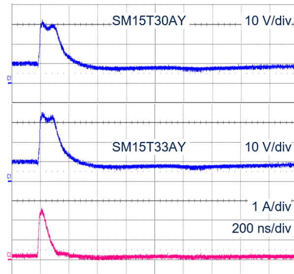
Figure 16. ISO7637-2 pulse 3b: V_s = +150 V with 12 V battery
