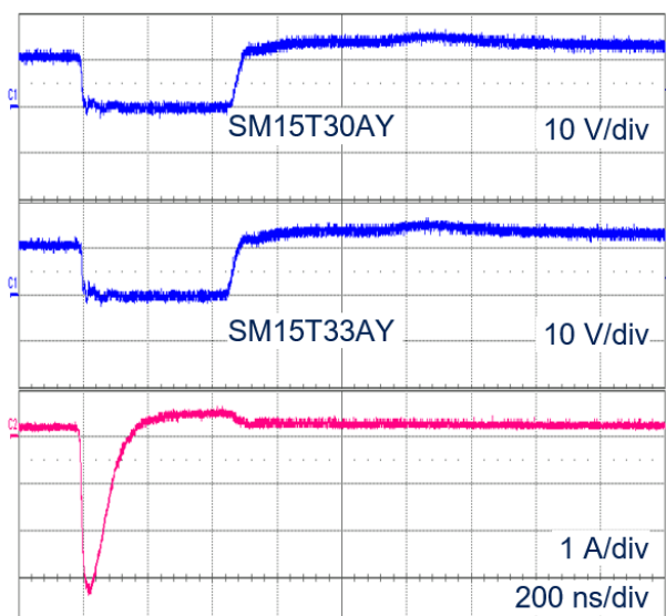
Figure 15. ISO7637-2 pulse 3a: V_s = -220 V with 12 V battery
