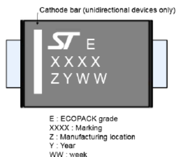
Figure 19. Marking layout
