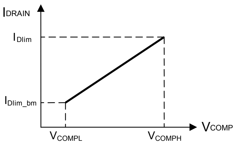
Figure 27. COMP pin voltage versus I_{DLIM}
