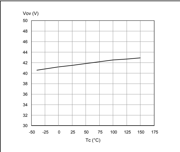
Figure 11. Overvoltage shutdown
