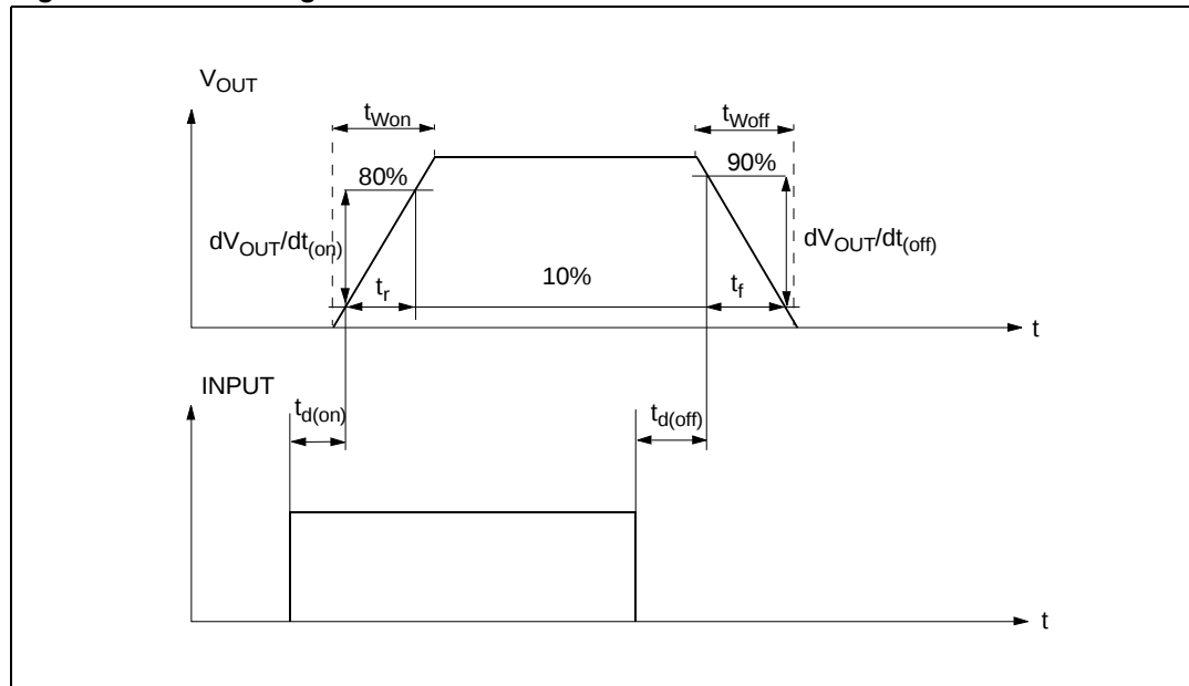
Figure 6. Switching characteristics
