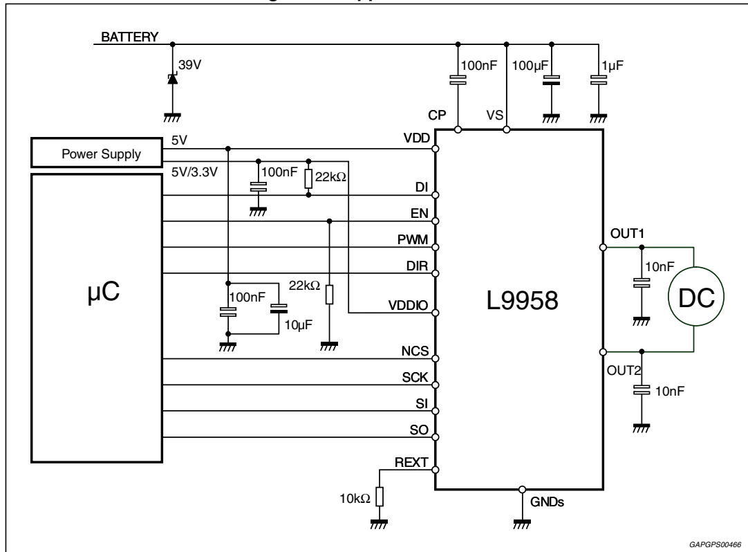
Figure 22. Application circuit
