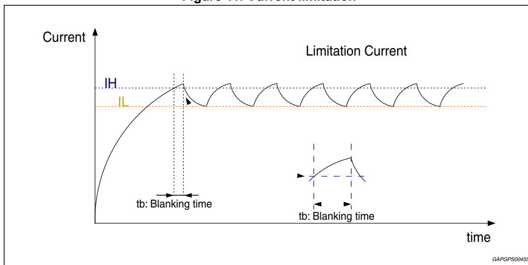
Figure 11. Current limitation
