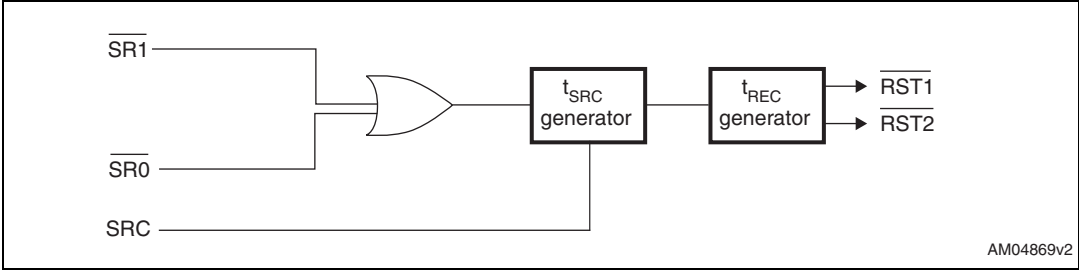
Figure 3. Block diagram
