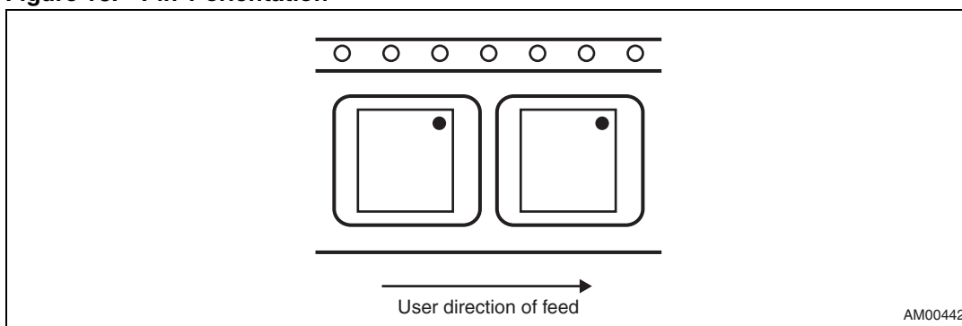
Figure 18. Pin 1 orientation
