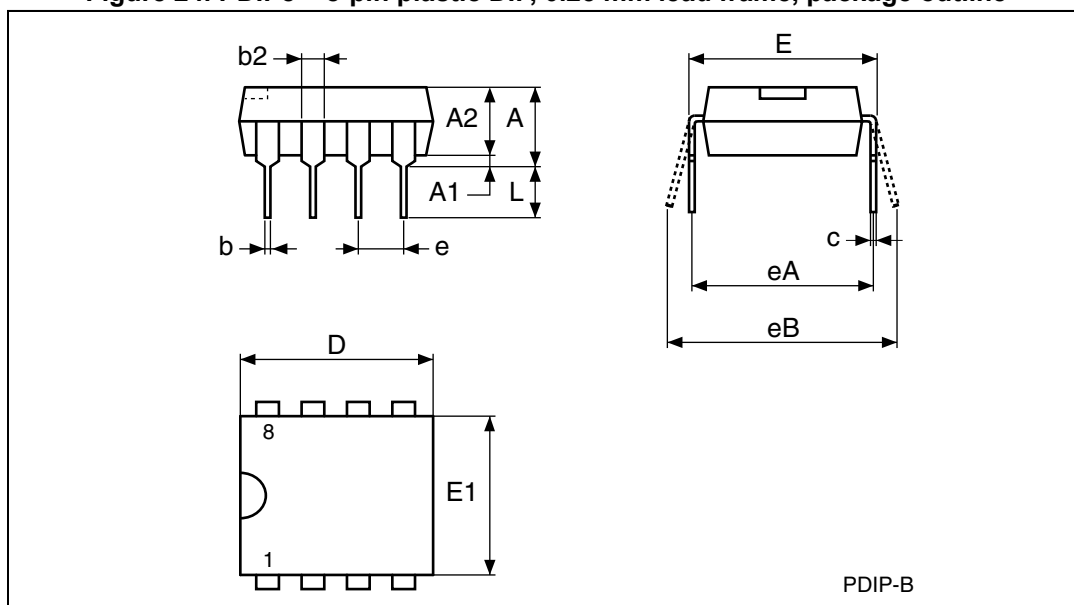
Figure 24. PDIP8 – 8-pin plastic DIP, 0.25 mm lead frame, package outline
