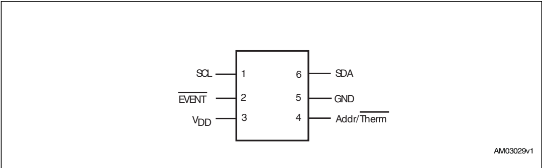
Figure 2. Pinout
