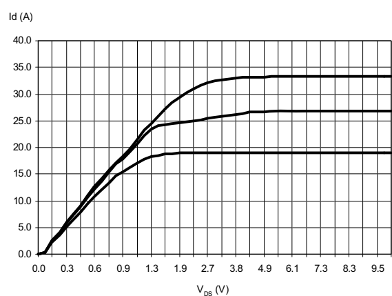
Figure 23. Output characteristics
