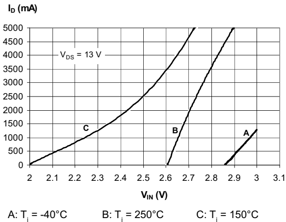
Figure 11. Transfer characteristics (inside view for V_{IN} = 2 V to 3 V)
