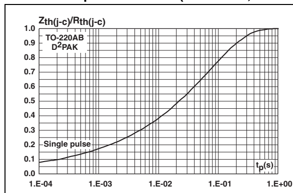
Figure 3. Relative variation of thermal impedance junction to case versus pulse duration (TO-220AB, D²PAK)
