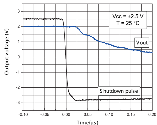
Figure 21. Turn-off time, V_{\text{CC}} = \pm 2.5 V, Vout pulled down, T = 25^\circ\text{C}
