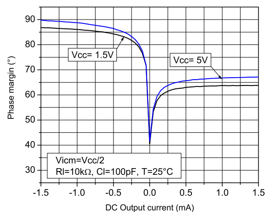
Figure 7. Phase margin vs. output current at V_{CC} = 1.5\text{ V} and V_{CC} = 5\text{ V}
