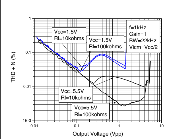
Figure 14. Distortion + noise vs. output voltage
