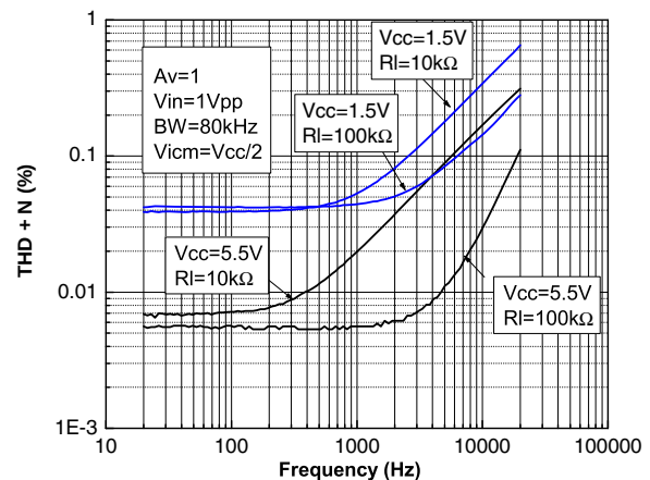
Figure 13. Distortion + noise vs. frequency
