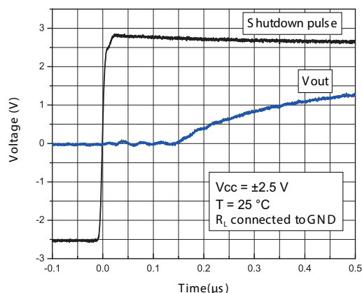
Figure 20. Turn-on time, V_{\text{CC}} = \pm 2.5 V, Vout pulled down, T = 25^\circ\text{C}
