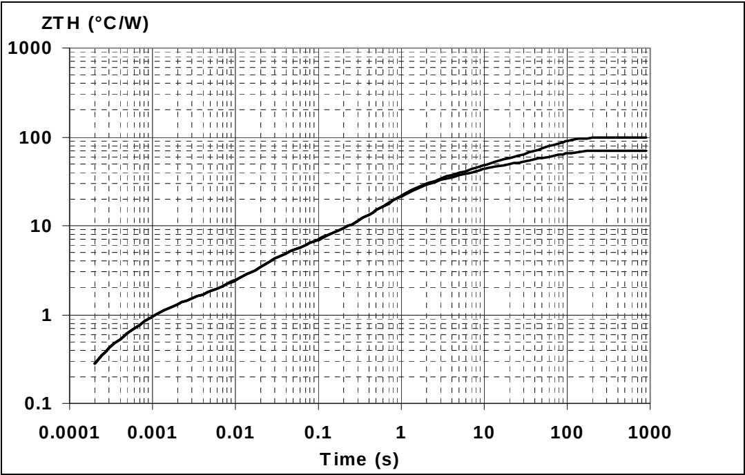
Figure 36. SO-8 thermal impedance junction ambient single pulse
