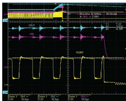
Figure 38. Output voltage ripple at 230 V IN_AC no load
