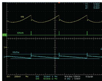
Figure 15. Output voltage ripple at 115 V IN_AC no load
