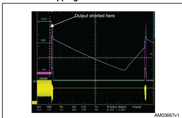
Figure 26. OLP: output short and protection tripping
