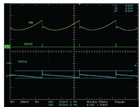
Figure 16. Output voltage ripple at 230 V IN_AC no load
