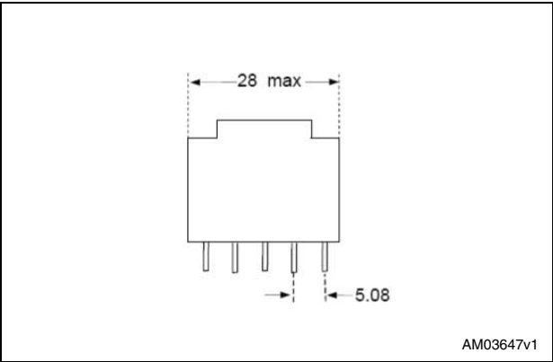
Figure 6. Transformer size - side view 2
