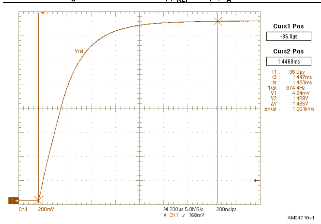
Figure 38. Reference startup, I_{REF} = 15\ \mu\text{F} , T_A = 25^\circ\text{C}
