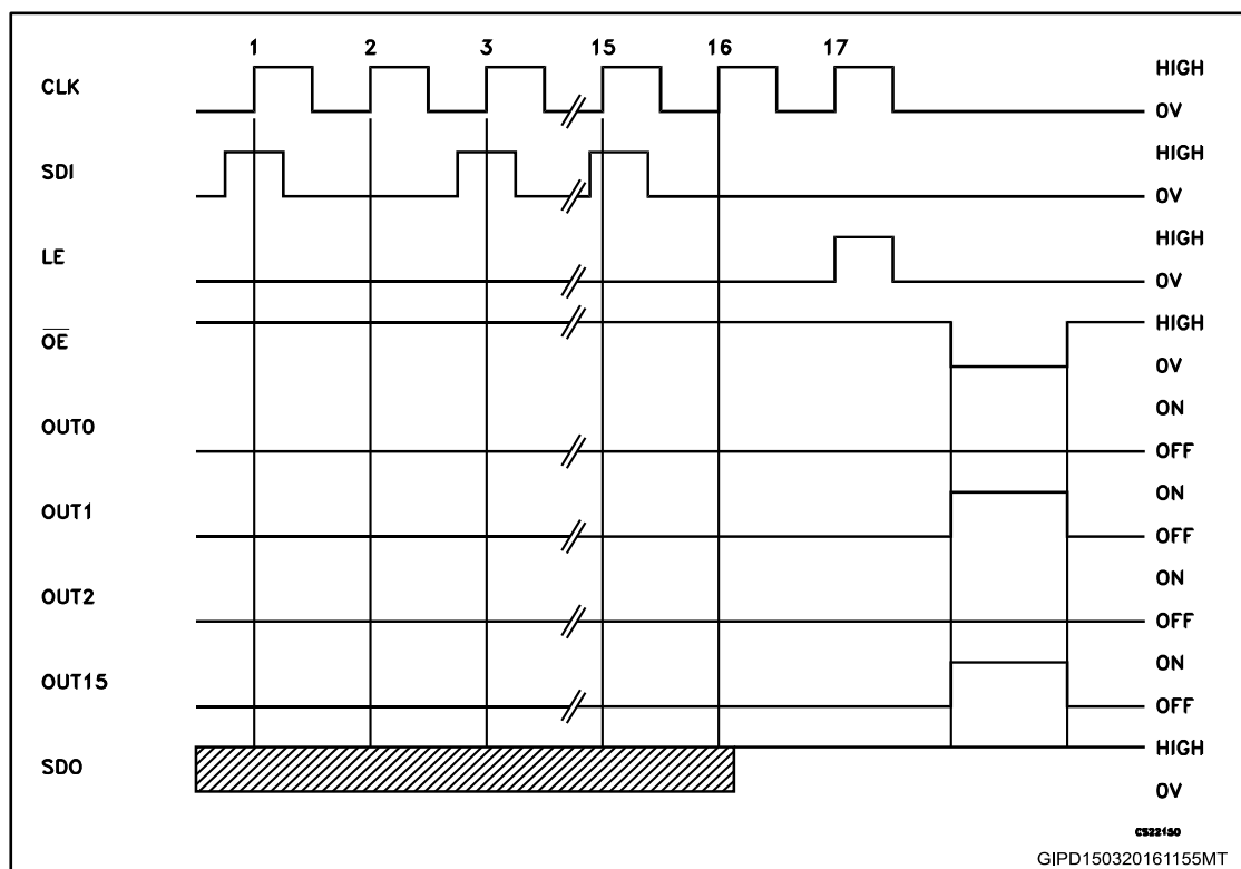
Figure 7: Timing diagram
