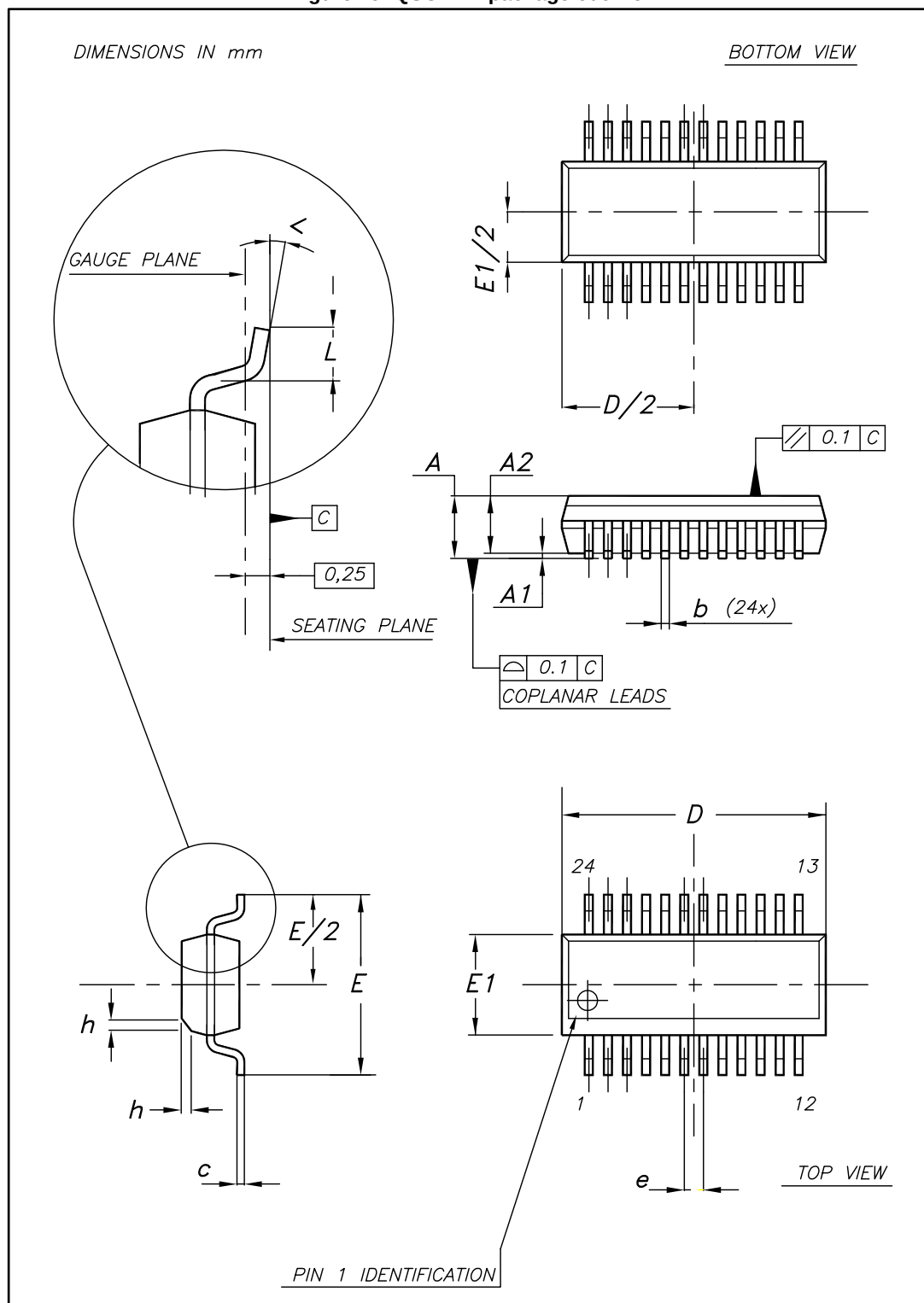
Figure 19: QSOP-24 package outline
