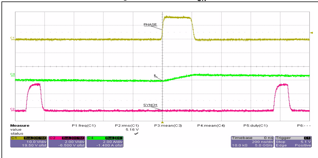
Figure 12. Minimum T_{ON}
