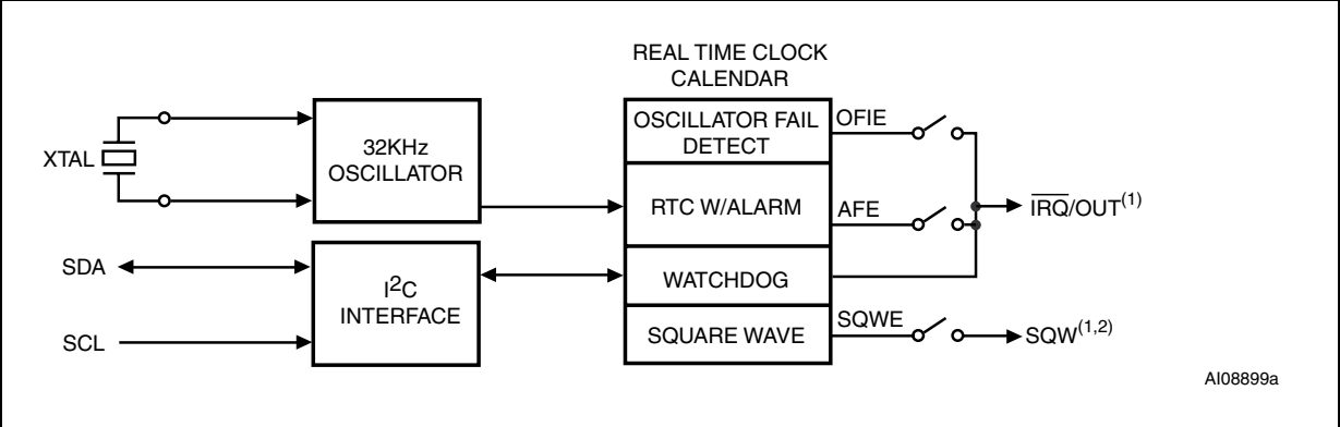
Figure 3. M41T66 block diagram
