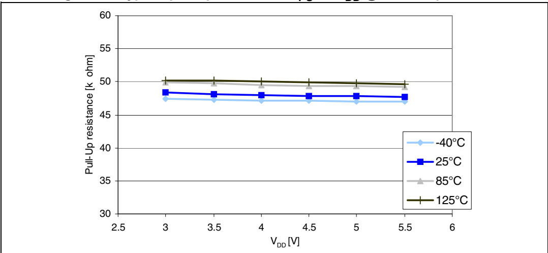
Figure 21. Typical pull-up resistance R_{PU} vs V_{DD} @ four temperatures
