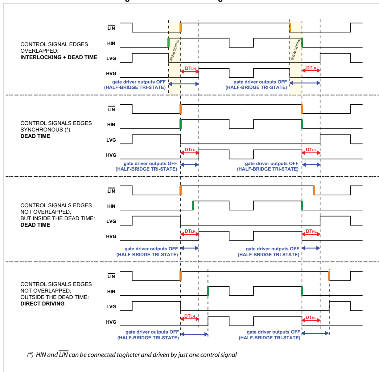
Figure 5. Deadtime - timing waveforms
