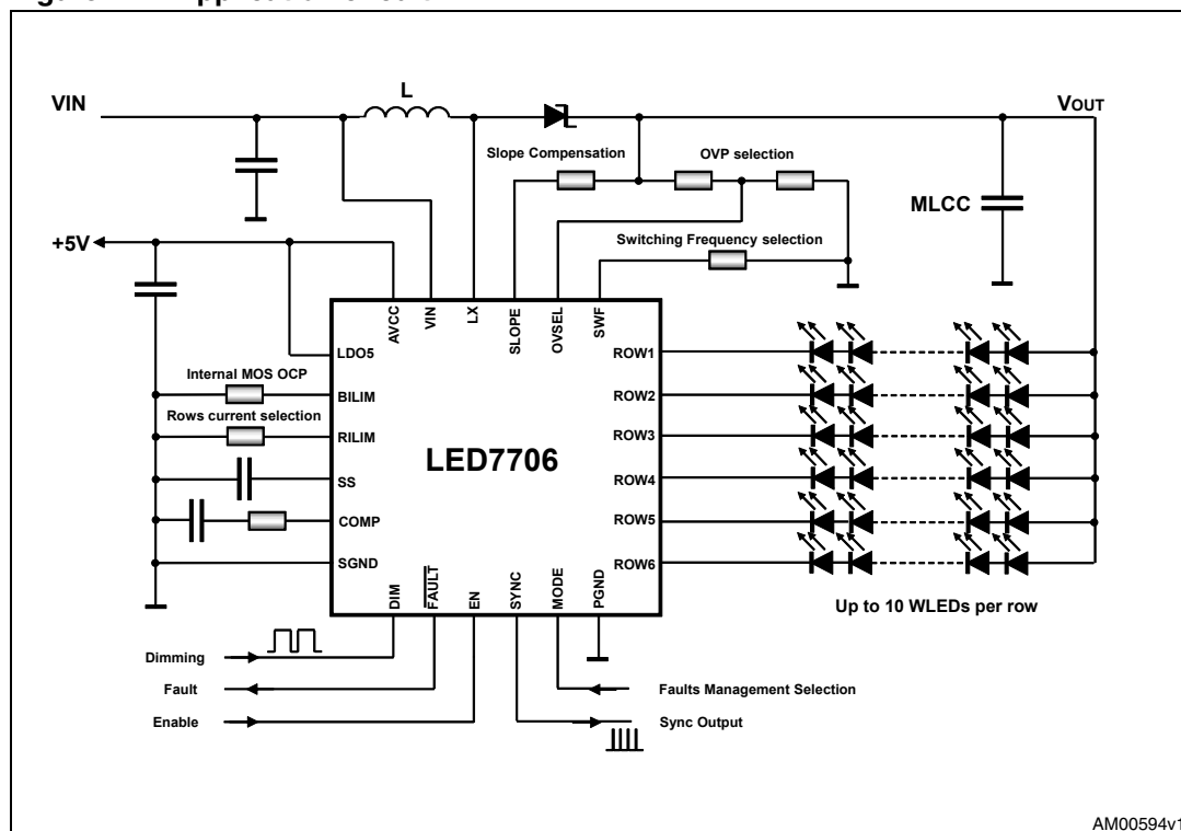
Figure 1. Application circuit
