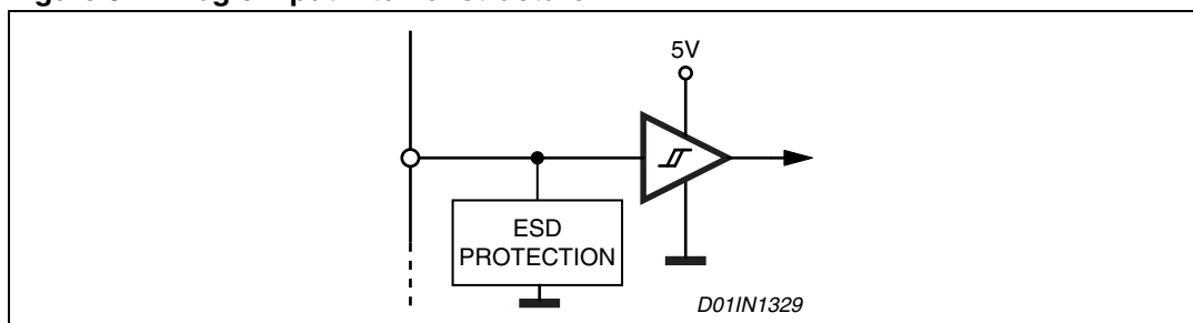
Figure 9. Logic input internal structure
