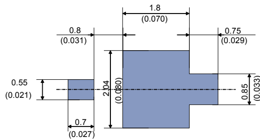
Figure 13. Footprint recommendations, dimensions in mm (inches)
