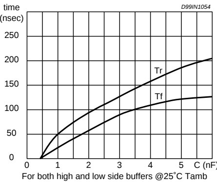
Figure 4. Typical rise and fall times vs. load capacitance
