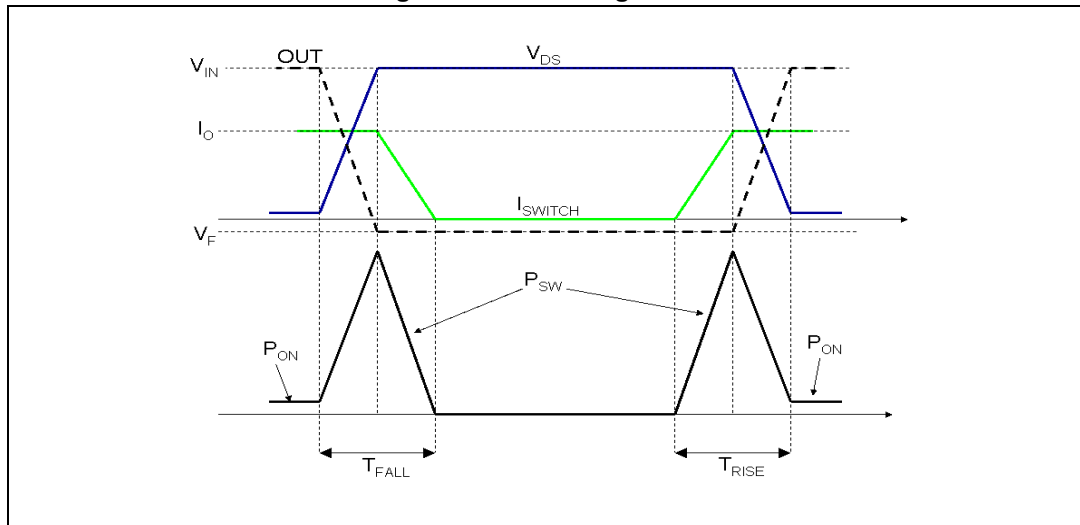
Figure 12. Switching losses
