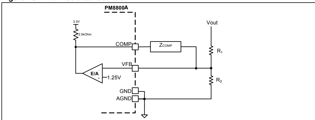
Figure 13. Non-isolated feedback
