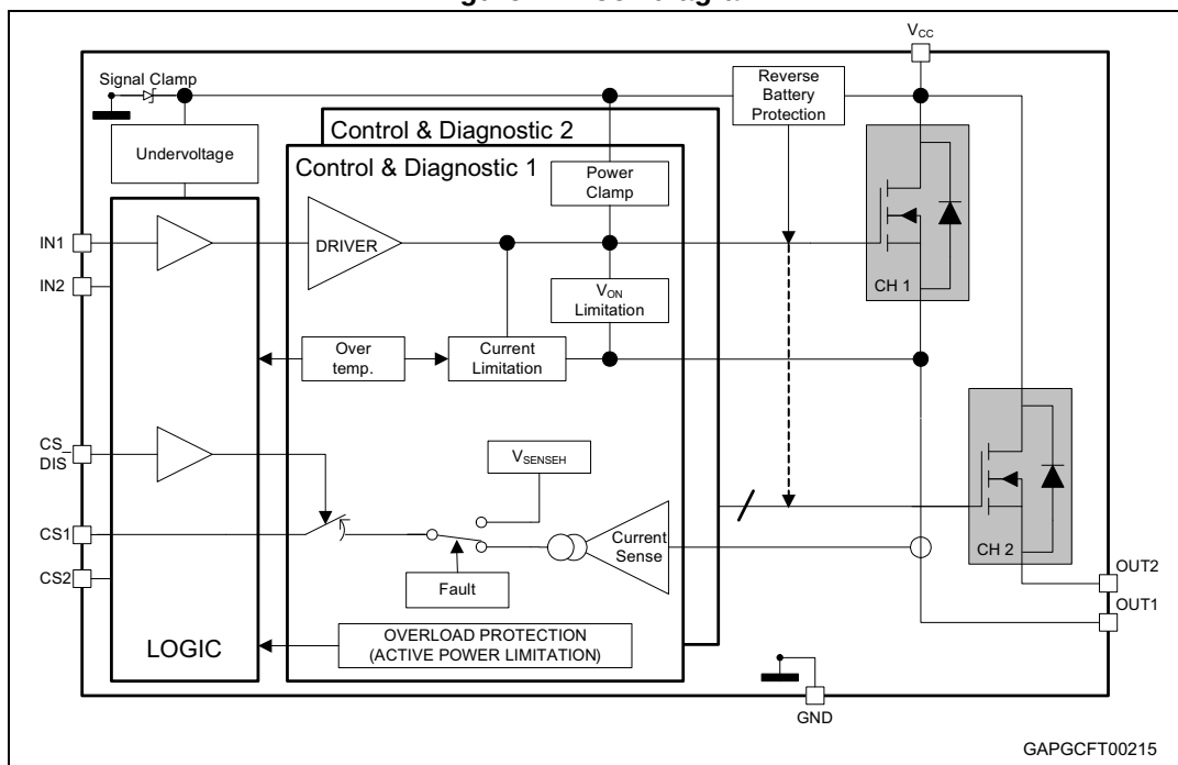
Figure 1. Block diagram
